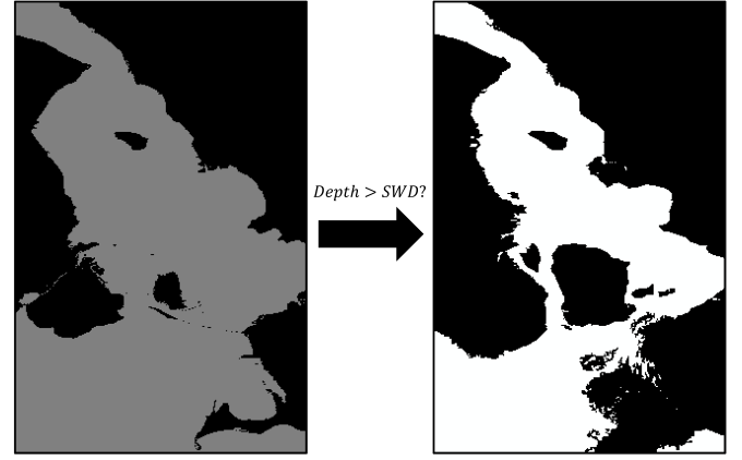
Fig. 5. Workflow for generating a binary navigability mask from EMODnet bathymetric data. (Left) High-resolution water depth raster derived from EMODnet. (Right) Binarized navigability mask classifying regions as navigable (white) or non-navigable (black) through thresholding at SWD ( SWD = Draft_{\max} + UKC_{\min} ). The arrow indicates the geospatial processing pipeline.
