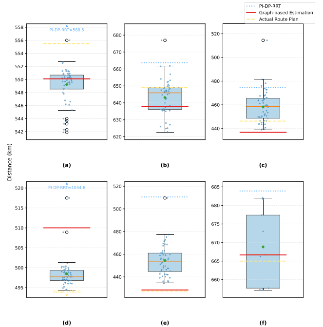
Fig. 13. Box-and-whisker plots of traveled distance for historical trajectories with similar origin and destination to OD1 to OD6. The boxes show the AIS historical distributions. Horizontal markers indicate the distances of the proposed framework, PI-DP-RRT, and (optionally) the VesselFinder plan. Panel titles (a–f) correspond to OD1–OD6.
