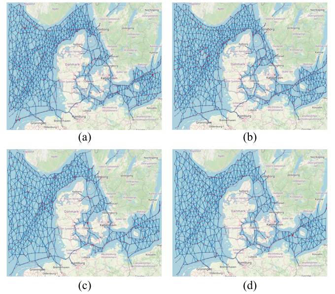
Fig. 8. Centroid points and flows derived from the tanker dataset through Algorithm 1 and Algorithm 2, employing different parameter configurations of d_{min} and d_{max} : (a) d_{min} = 3 km, d_{max} = 20 km. (b) d_{min} = 4 km, d_{max} = 20 km. (c) d_{min} = 3 km, d_{max} = 25 km. (d) d_{min} = 4 km, d_{max} = 25 km.
