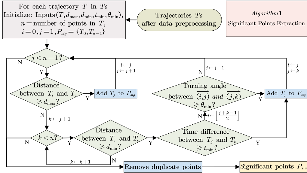
Fig. 1. Flowchart for extracting significant points from AIS tracks. Besides trajectories' start and end points, P_{\text{sig}} includes three types of significant points: significant distance points P_{sd} where the distance from the previous point exceeds d_{\max} , significant turning points P_{st} where the turning angle exceeds \theta_{\min} , and significant stopping points P_{ss} where the stop duration within a certain area exceeds t_{\min} .
