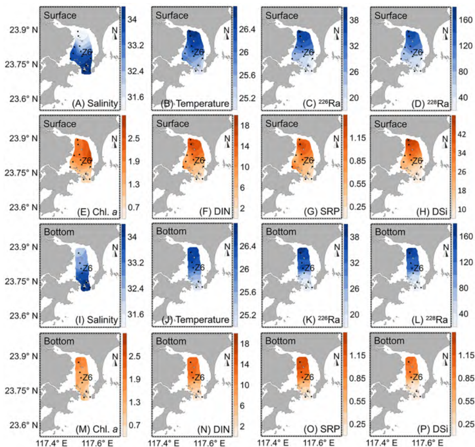
FIGURE 4 Distribution of salinity, temperature (°C), radium isotopes (dpm 100 L -1 ), Chl. a (µg L -1 ), and nutrients (µmol L -1 ) in Dongshan Bay on 28 May 2020. (A–H) surface water and (I–P) bottom water.
