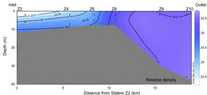
FIGURE 5 The sectional distribution of the density (kg m -3 ) anomaly from the inlet to the outlet in Dongshan Bay on 28 May 2020. The figure was produced using Ocean Data View v. 5.6.2 ( https://odv.awi.de ).
