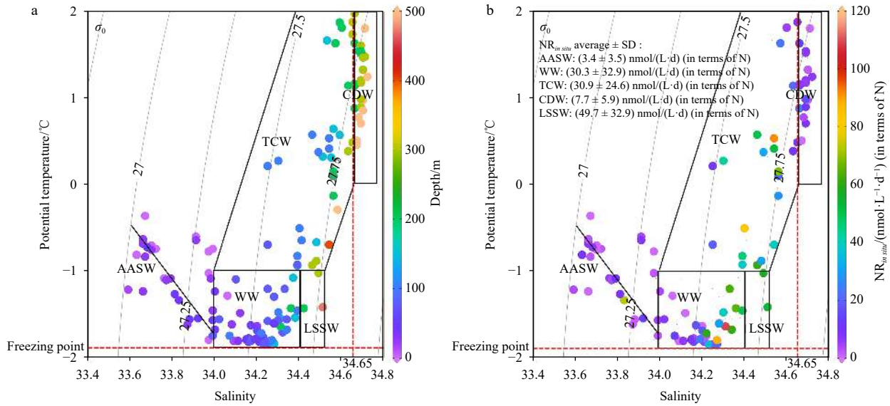
Fig. 2. In-situ nitrification rates in different water masses above 500 m depth. a. Potential temperature ( \theta ) versus salinity at sampling sites. The light grey curves represent the contours of potential density anomalies referenced to zero pressure ( \text{kg/m}^3 ). The dashed red lines along the x- and y-axes represent the surface freezing point ( -1.89^\circ\text{C} ) and the salinity 34.65 contours. The water masses in the upper 500 m include Antarctic Surface Water (AASW), Winter Residual Water (WW), Thermocline Water (TCW), Circumpolar Deep Water (CDW), and Low-Salinity Shelf Water (LSSW). The characteristic range of potential temperature and salinity for each water mass is marked with black rectangles and lines. The detailed information and classification of water masses are given in the Text S1. b. The in situ nitrification rate [ \text{NR}_{in\ situ} nmol/(L·d), in terms of N] in each water mass, its average \pm standard deviation (SD) is shown in the upper left corner.
