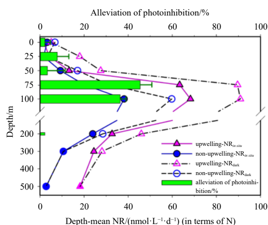
Fig. 10. Depth-averaged profiles of nitrification rate in situ ( NR_{in situ} ) and in darkness ( NR_{dark} ) and photoinhibition alleviation between upwelling and non-upwelling sites. NR_{in situ} for upwelling and non-upwelling sites are indicated by solid pink triangles and solid blue circles, respectively. NR_{dark} for upwelling and non-upwelling sites are indicated by open triangles and circles, respectively. The percent alleviation from photoinhibition calculated from the difference between the percent inhibition of upwelling and non-upwelling sites is represented by green horizontal bars with dark green error bars. Note that a break is set at a depth of 122 m for better visualization.
