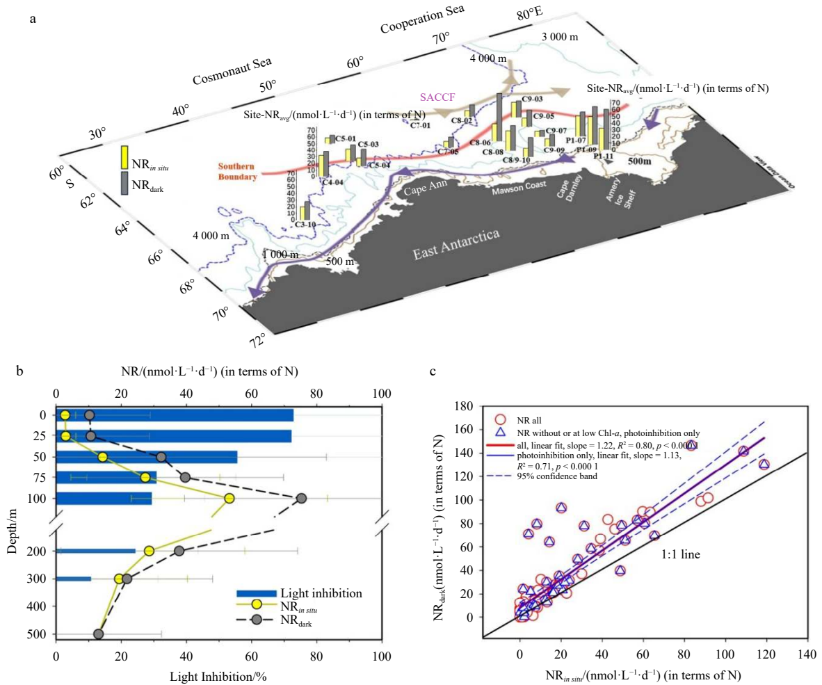
Fig. 5. Light inhibition on nitrification. a. Spatial variation of site averages of nitrification rates ( NR_{avg} , nmol/(L·d), in terms of N) under in situ (yellow bar) and dark conditions (grey bar). The brown, red, and purple lines show the Southern Antarctic Circumpolar Current (ACC) Front (SACCF, 1.8 °C isotherm), Southern Boundary of ACC (SB, 1.5 °C isotherm), and Antarctic Slope Current, respectively. b. Profiles of mean NR_{in situ} (yellow dots) and NR_{dark} (dark grey dots) at depth are shown with their respective error bars for all sites. The Light Inhibition calculated from the difference between mean NR_{in situ} and NR_{dark} is represented by horizon blue bars with light blue error bars. Note that a break is set at a depth of 122 m for better visualization. c. The relationship between NR_{in situ} and NR_{dark} under paired incubation experiments. The linear fit equation (red circles and dark red line) has a slope of 1.22, and the linear fit equation (blue triangles and dark blue line with 95% confidence band between double dashed blue lines) has a slope of 1.13 at low chlorophyll a (Chl- a ) levels. The black solid line represents the 1:1 line.
