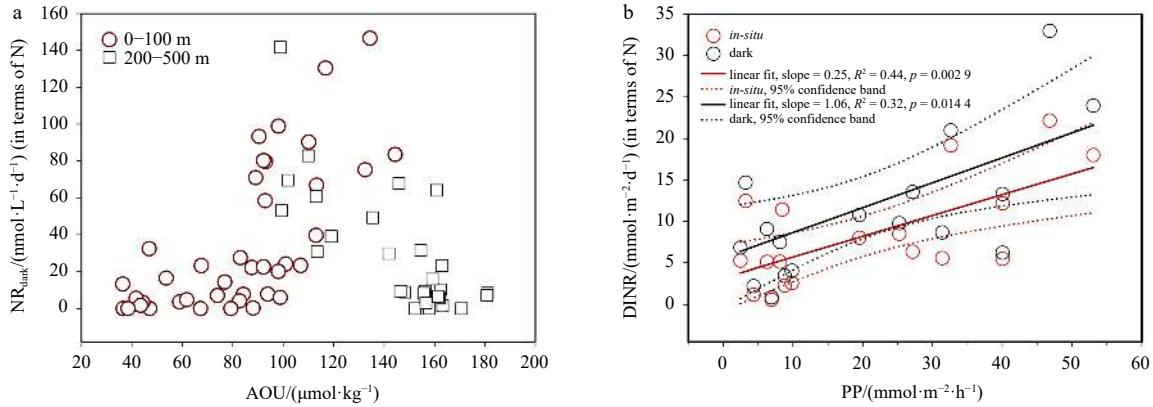
Fig. 6. The relationship between on-site nitrification rate and environmental factors. a. Relationship between nitrification rate in darkness ( NR_{dark} ) and apparent oxygen consumption (AOU). The NR_{dark} in the upper 100 m water column increases exponentially with the increase of AOU (dark red circle). No correlation was observed between the two at the depth of 200–500 m due to the low available substrate (black square). b. Relationship between depth-integrated nitrification rate (DINR) and primary productivity (PP). Results in situ and the dark are shown in red and black, respectively.
