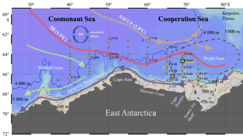
Fig. 1. Sampling locations, bathymetry, and circulation in the Indian sector of the Southern Ocean, 62°–68°S and 30°–80°E. Sections C3, C4, C5, C6, and C7 are located in the Cosmonaut Sea, and Sections C8, C9, and P1 are located in the Cooperation Sea. All dots represent CTD observation and nutrient sampling sites. Yellow dots indicate nitrification rate measurements in situ and in the dark. The two yellow underlines indicate sites where substrate kinetic experiments for nitrification under light and dark conditions were performed. Oceanographic features highlighted include the Southern Antarctic Circumpolar Current Front (SACCF, 1.8°C isotherm, brown line), the Southern Boundary of the upper CDW (SB, 1.5°C isotherm, red line), and the Antarctic Slope Current (purple line) (Orsi et al., 1995). Dark blue circular arrows indicate the Antarctic Divergence zone (AD) between the SACCF and SB, with a large number of mesoscale eddies (Talley et al., 2011). The eastern boundary of the Weddell Gyre is marked by a green line with an arrow. The Prydz Bay Gyre is marked by a gray dashed circle (Heywood et al., 1999). The location of the Cape Darnley Polynas (CDP) is marked off the Mawson Coast. The isobaths at 500 m, 1 000 m, 3 000 m, and 4 000 m are represented by khaki, black dashed, turquoise, and blue lines, respectively.
