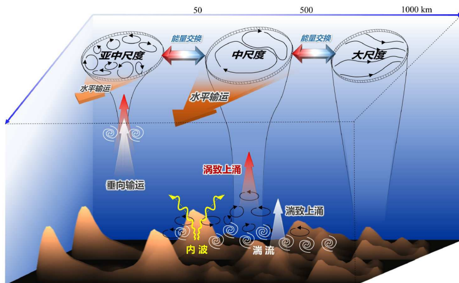
图3 海洋中小尺度动力过程及其物质能量输运与气候效应 Figure 3 Transportation of energy and materials and climatic effects of meso- and submesoscale oceanic processes
