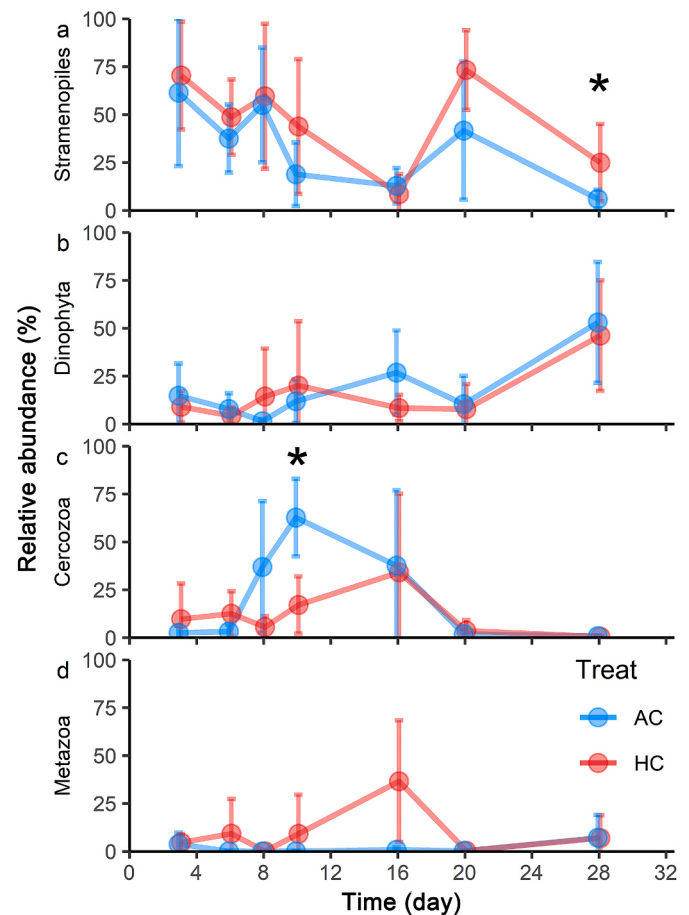
Fig. 3. Relative abundance of the most abundant microeukaryotic phyla under high \text{CO}_2 (HC) and ambient \text{CO}_2 (AC) throughout the experiment: Stramenopiles (a), Dinophyta (b), Cercozoa (c) and Metazoa (d). Data are means \pm SD of replicates for HC treatments and for AC treatments. *Indicates significant difference between HC and AC at that time point ( P < 0.05 ).
