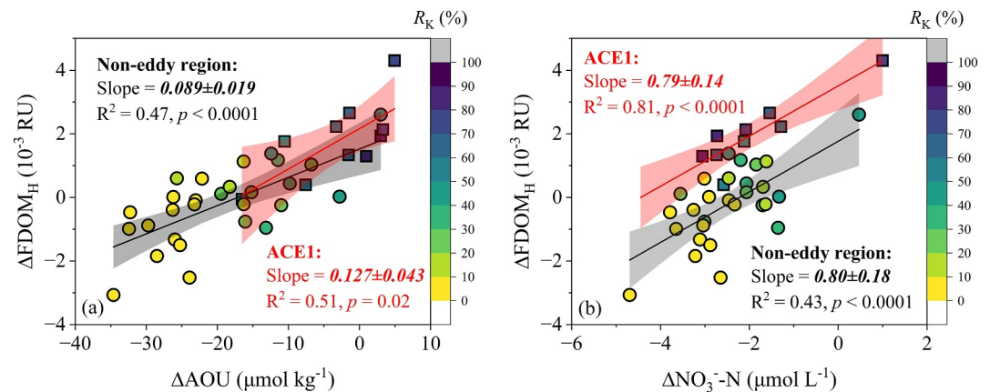
Figure 5. Relationships between \Delta\text{FDOM}_H (represented by peak M) with \Delta\text{AOU} , \Delta\text{NO}_3^-N in anticyclonic eddy ACE1 (squares, 150–250 m) and non-eddy region (circles, 150–300 m). The color bar indicates the Kuroshio water fraction. The occurrence of negative \Delta\text{FDOM}_H , \Delta\text{AOU} and \Delta\text{NO}_3^-N values are possibly due to their low values in the premixing water masses compared to those in the endmembers of the mixing model.
