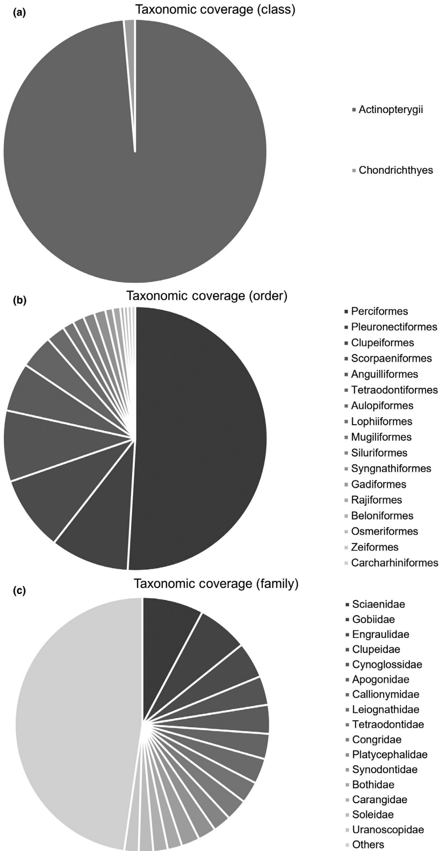
FIGURE 7 Taxonomic coverage of feed-grade fish samples. (a) Class, (b) order and (c) family
