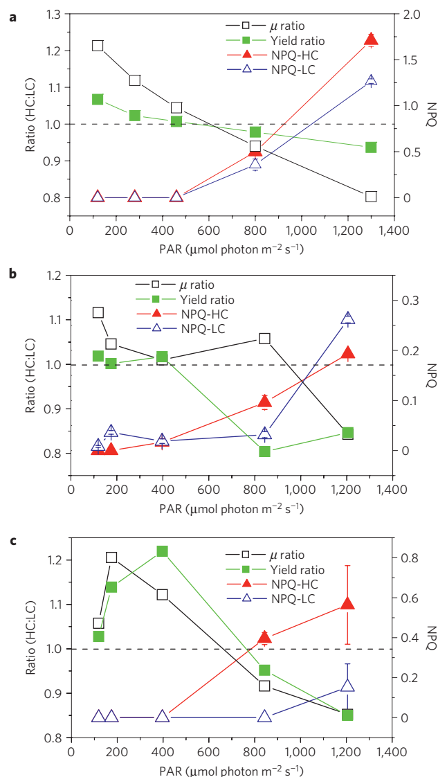
Figure 3 | High- to low- p\text{CO}_2 ratios for growth rates and photosynthetic parameters in cultured diatoms. a–c. The ratios of \mu (open square) and effective yields (green filled square) in high- \text{CO}_2 -grown cells (HC, 1,000 \mu\text{atm} ) to those in low- \text{CO}_2 -grown cells (LC, 390 \mu\text{atm} ), and their NPQ (red filled triangle for HC and blue open triangle for LC) in the diatoms, Phaeodactylum tricornutum (a), Thalassiosira pseudonana (b) and Skeletonema costatum (c), as a function of PAR levels, equivalent to solar PAR levels during noon period for the same cultures grown outdoors (Fig. 2). Note, both growth rate and yield reversed with increased PAR levels and NPQ increased faster with increased PAR levels in the high- \text{CO}_2 -grown cells.
