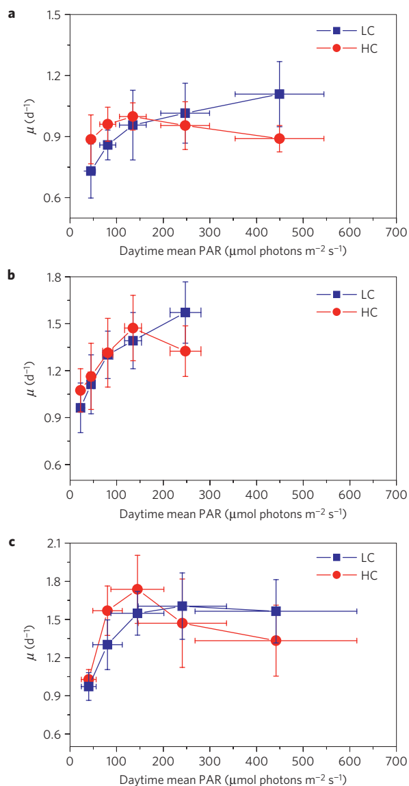
Figure 2 | Growth rates of cultured diatoms as a function of p\text{CO}_2 and light. a–c. \mu of the diatoms Phaeodactylum tricornutum (a), Thalassiosira pseudonana (b) and Skeletonema costatum (c) grown under ambient (390 \mu\text{atm} , LC, blue square) and increased \text{CO}_2 (1,000 \mu\text{atm} , HC, red circle) conditions under 5%, 10%, 18%, 30%, 55% or 100% levels of incident sunlight for P. tricornutum (December 2010) and 5%, 10%, 18%, 30% and 55% for T. pseudonana (March 2011) and S. costatum (April 2011). Each symbol represents the average of six replicate cultures under each treatment. Seawater carbonate system parameters are given in Supplementary Table S1. Horizontal and vertical error bars denote standard deviations for variation of solar radiation and \mu , respectively.
