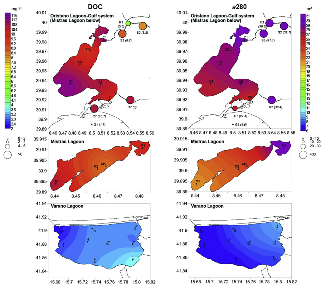
Fig. 2. Spatial distribution of DOC and absorption coefficients at 280 nm ( a_{280} ) in the surface waters of the Oristano Lagoon-Gulf (OLG) system and the Varano Lagoon (sampling date: 9 September 2014). In OLG, values at the riverine and Gulf sites are also indicated in parentheses.
