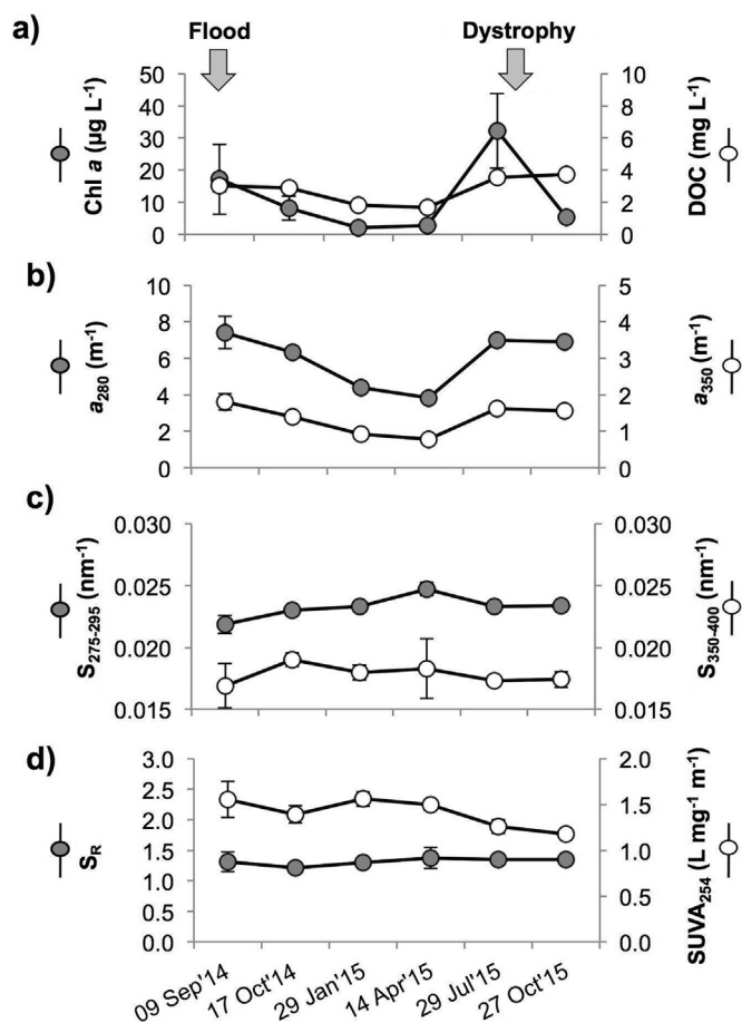
Fig. 4. Monthly variations (mean \pm SD, n = 9 ) in trophic (Chlorophyll a and dissolved organic carbon) and optical variables in the Varano Lagoon: a) chlorophyll a (Chl a ) and dissolved organic carbon (DOC); b) absorption coefficients at 280 nm and 350 nm ( a_{280} and a_{350} ); c) spectral slopes in the ranges 275–295 nm and 350–400 nm ( S_{275-295} and S_{350-400} ), their slope ratio ( S_R ) and organic matter aromaticity ( \text{SUVA}_{254} ). The arrows indicate the time of occurrence of the flood and the dystrophic event.
