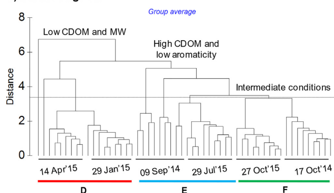
Fig. 6. a, b. Cluster diagram based on trophic (Chlorophyll a and dissolved organic carbon) and chromophoric dissolved organic carbon (CDOM) optical variables for a) the Oristano Lagoon-Gulf system (15 sampling sites, G1 and sediment pore-water excluded); and b) the Varano Lagoon (9 sampling sites \times 6 sampling dates). MW = molecular weight.
