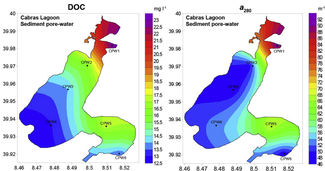
Fig. 3. Spatial distribution of DOC and absorption coefficients at 280 nm ( a_{280} ) in the sediment pore-water of Cabras Lagoon (note the different scale from Fig. 2).
