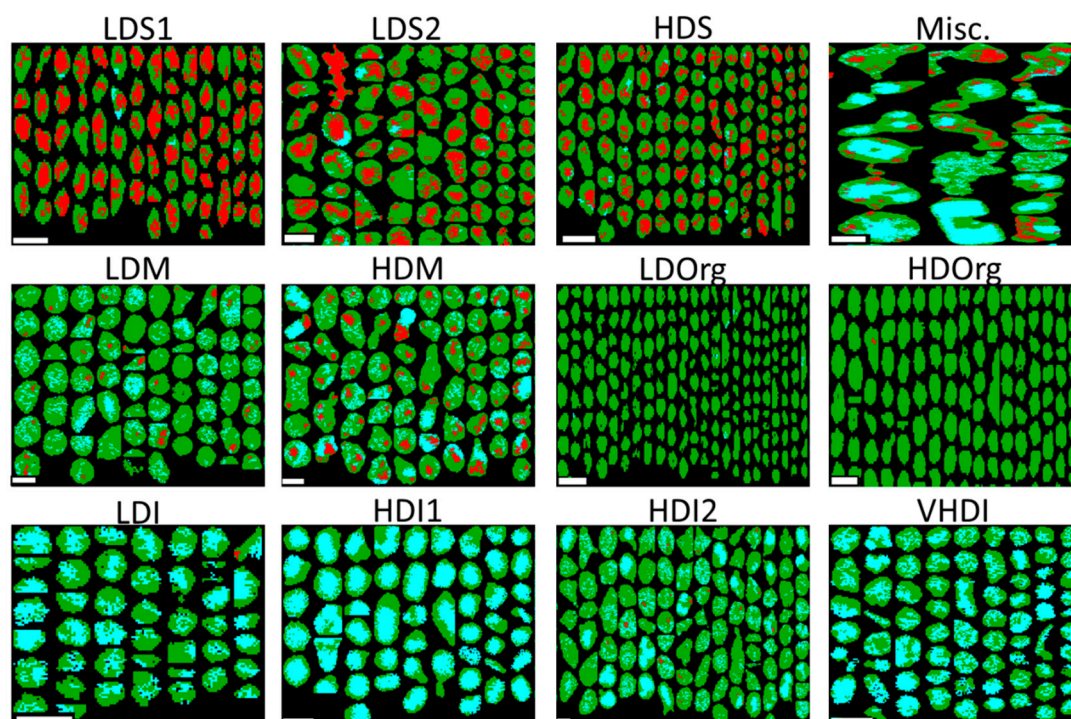
Figure 3. Random sample of \sim 40 particles from each cluster showing sub-particle carbon speciation as either soot (red), inorganic (teal), or organic (green). 1 \mu\text{m} scale bars are shown in the bottom left of each image. Cluster identification (image labels) is provided in Table 3.
