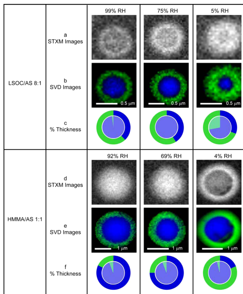
Figure 2. STXM data for LSOC/AS 8:1 OIR (a–c) and HMMA/AS 1:1 OIR (d–f) at high RH (left column), intermediate RH (middle column) and low RH (right column). STXM images at 288.5 eV (a and d). Singular value decomposition images with inorganic (blue) and organic (green) regions (b and e). Fraction of thickness due to organic (green) and inorganic (blue) (c and f). The inner circle (lighter colors) corresponds to the organic versus inorganic fractions in the center of the particles and the outer circle (darker colors) corresponds to the fractions of organic and inorganic components in the particle edge.
