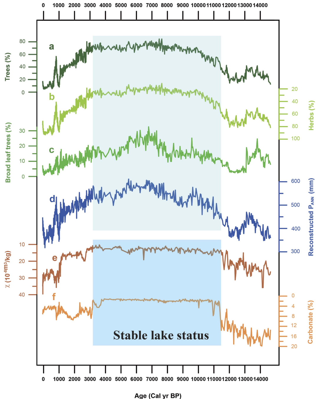
Figure 2. Variation in the reconstructed annual precipitation and other environmental proxies since 14.7 ka from Gonghai Lake, North China. (a) Percentage of tree pollen (%). (b) Percentage of herb pollen (%). (c) Percentage of broad leaf tree pollen (%). (d) Annual precipitation reconstructed by a calibration function applied to the fossil pollen assemblages. (e) Magnetic susceptibility. (f) Carbonate content. Shaded area from ~11.5–3.3 ka denotes an interval of stable lake status and maximum vegetable cover in the Gonghai Lake catchment.
