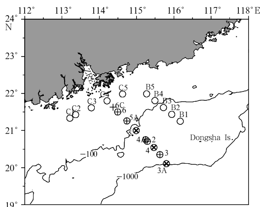
Fig.1. CTD and sampling stations in the northern South China Sea. +: CTD and sampling stations in May 2001; x: stations only for CTD in May 2001; o: CTD and sampling stations in November 2002; ZRE: the Zhujiang River Estuary; Dongsha Is.: Dongsha Island.
