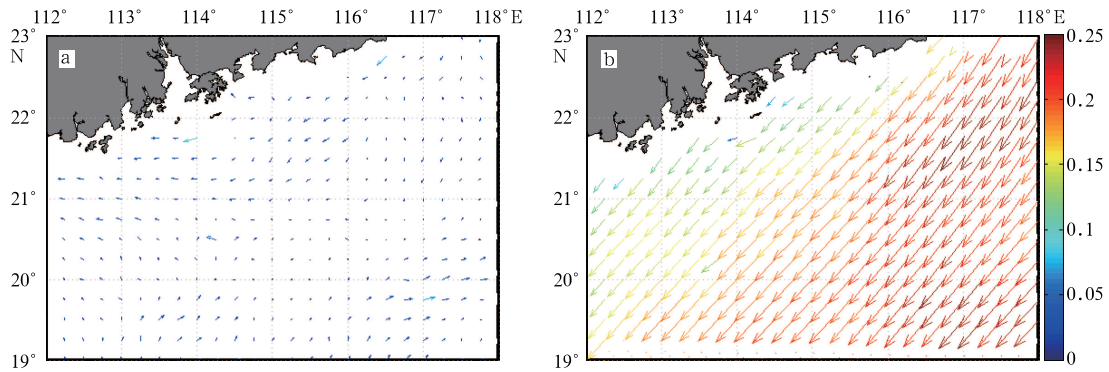
Fig.7. Monthly mean wind stress as observed by QuikSCAT during May 2001 (a) and November 2002 (b). The unit is \text{N/m}^2 .
