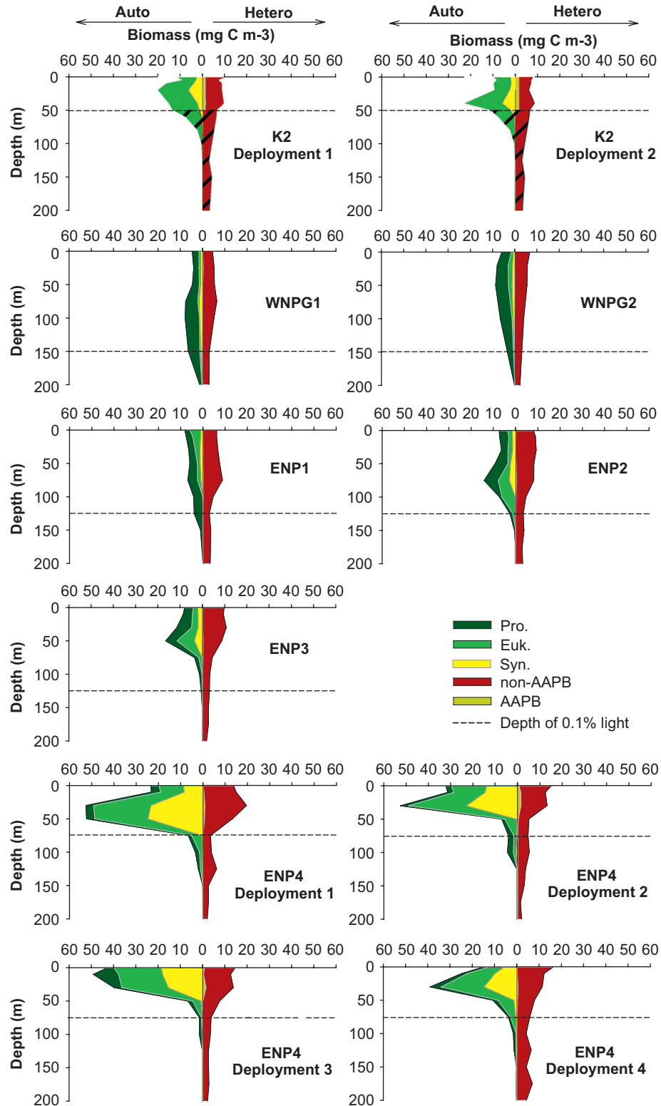
Fig. 3. Depth profiles of picoplankton carbon biomass (X-axis: autotrophic-left and heterotrophic-right of zero) in the subarctic area (K2), the Western North Pacific subtropical gyre (WNPG1–2) and the Eastern North subtropical Pacific (ENP1–4). In order to obtain complete vertical profiles of picoplankton carbon biomass at K2, data from 50 to 200 m (shaded) were fitted by including the results of a near-K2 station at 50°N 163°E during our Bering Sea cruise in July 2003. Pro.: Prochlorococcus ; Syn.: Synechococcus ; Euk.: picoeukaryotes. non-AAPB: other heterotrophic bacteria excluding AAPB.
