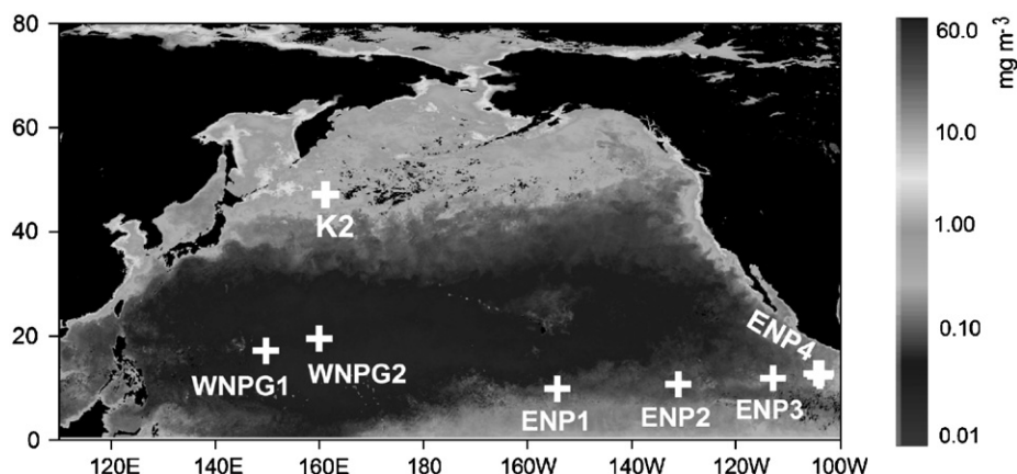
Fig. 1. Location of the sampling stations (crosses) in the North Pacific Ocean. The background chlorophyll a remote image (Aqua-MODIS) of August 2005 was downloaded from the website ( http://oceancolor.gsfc.nasa.gov/ ). Chlorophyll a scale shown on right in \text{mg m}^{-3} .
