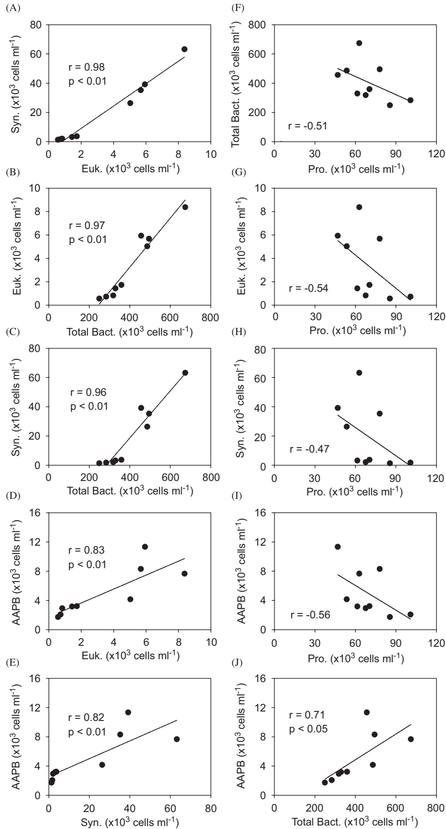
Fig. 4. Relationships between different groups of picoplankton. (A) Synechococcus vs. picoeukaryotes; (B) picoeukaryotes vs. bacteria; (C) Synechococcus vs. bacteria; (D) AAPB vs. picoeukaryotes; (E) AAPB vs. Synechococcus ; (F) bacteria vs. Prochlorococcus ; (G) picoeukaryotes vs. Prochlorococcus ; (H) Synechococcus vs. Prochlorococcus ; (I) AAPB vs. Prochlorococcus ; (J) AAPB vs. bacteria. Abundance data are depth-weighted averages over the euphotic zone. Pro.: Prochlorococcus ; Syn.: Synechococcus ; Euk.: picoeukaryotes; Total Bact.: total heterotrophic bacteria.
