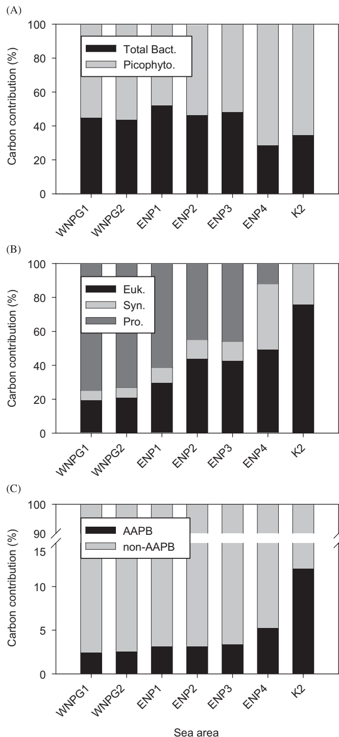
Fig. 5. Contribution of different groups of picoplankton to carbon biomass in the subarctic area (K2), the Western North Pacific subtropical gyre (WNPG1–2) and the Eastern North subtropical Pacific (ENP1–4). (A), total heterotrophic bacteria (Total Bact.) vs. pico-sized phytoplankton (picophyto.); (B), picoeukaryotes (Euk.) vs. Synechococcus (Syn.) vs. Prochlorococcus (Pro.); (C), AAPB vs. non-AAPB (other heterotrophic bacteria excluding AAPB). Values are % of carbon biomass of picoplankton calculated by depth-weighted average over euphotic zone.
