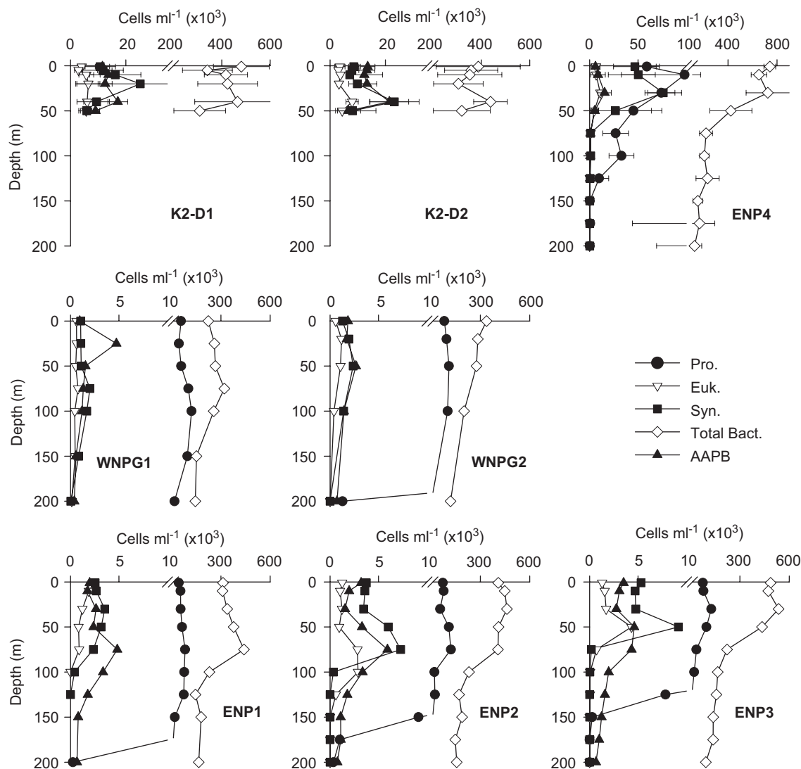
Fig. 2. Depth profiles of picoplankton abundance in the subarctic area (K2), the Western North Pacific subtropical gyre (WNPG1–2) and the Eastern North subtropical Pacific (ENP1–4). Error bars indicate standard deviation. Values of SD were calculated from the data of samples from four CTD casts each deployment at K2 and at ENP4. Note different X-axes are used. Pro.: Prochlorococcus ; Syn.: Synechococcus ; Euk.: picoeukaryotes; Total Bact.: total heterotrophic bacteria.
