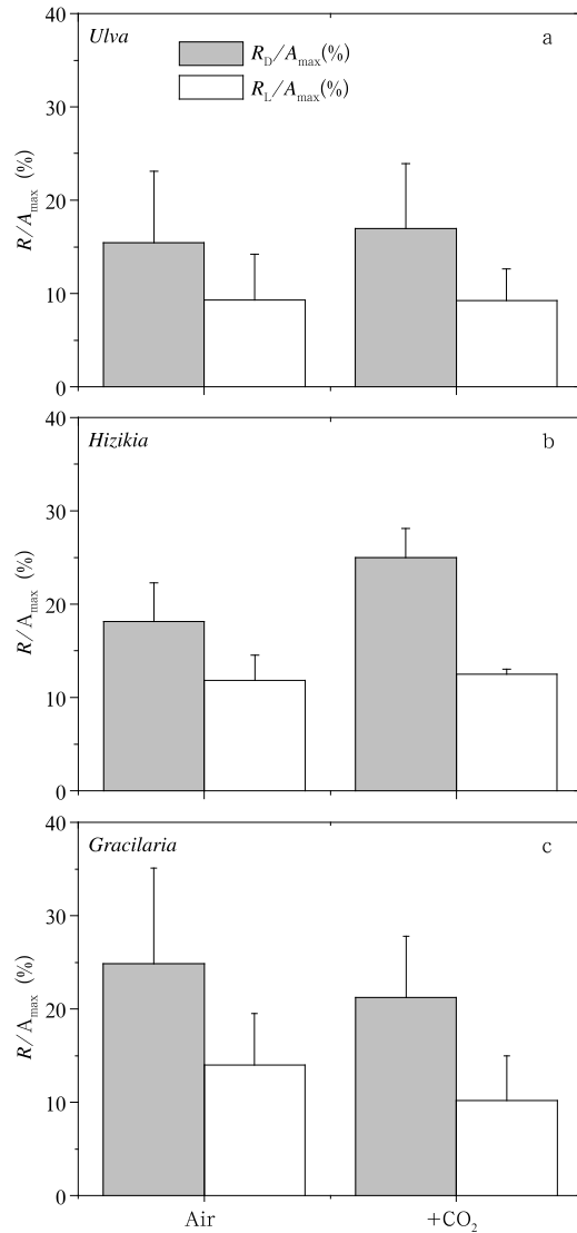
Fig.4. Percentage of R_L and R_D relative to light-saturating maximum net photosynthesis ( A_{max} ) in Ulva lactuca (a), Hizikia fusiformis (b) and Gracilaria lemaneiformis (c) cultured in seawater with aeration of ambient (Air) or CO 2 -enriched air (+CO 2 ). Vertical bars represent \pm SD of the means ( n=3 ).
