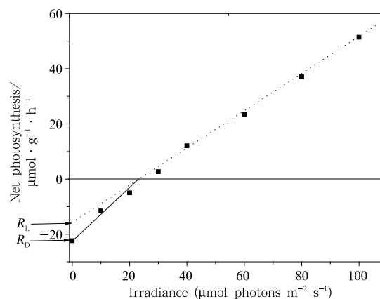
Fig.1. A representative example of photosynthetic light-response curve at low irradiance. The data are from Hizikia fusiformis grown at current ambient \text{CO}_2 . The linear regression section of light-response curve before the distinct break in the slope extrapolated back to the Y axis, and the intercept was given an estimate of dark respiration in the light ( R_L ), according to the Kok method. The value for the dark respiration in darkness ( R_D ) was taken at zero irradiance. The inflection in the slope of the curves occurs at the vicinity of the light compensation point.
