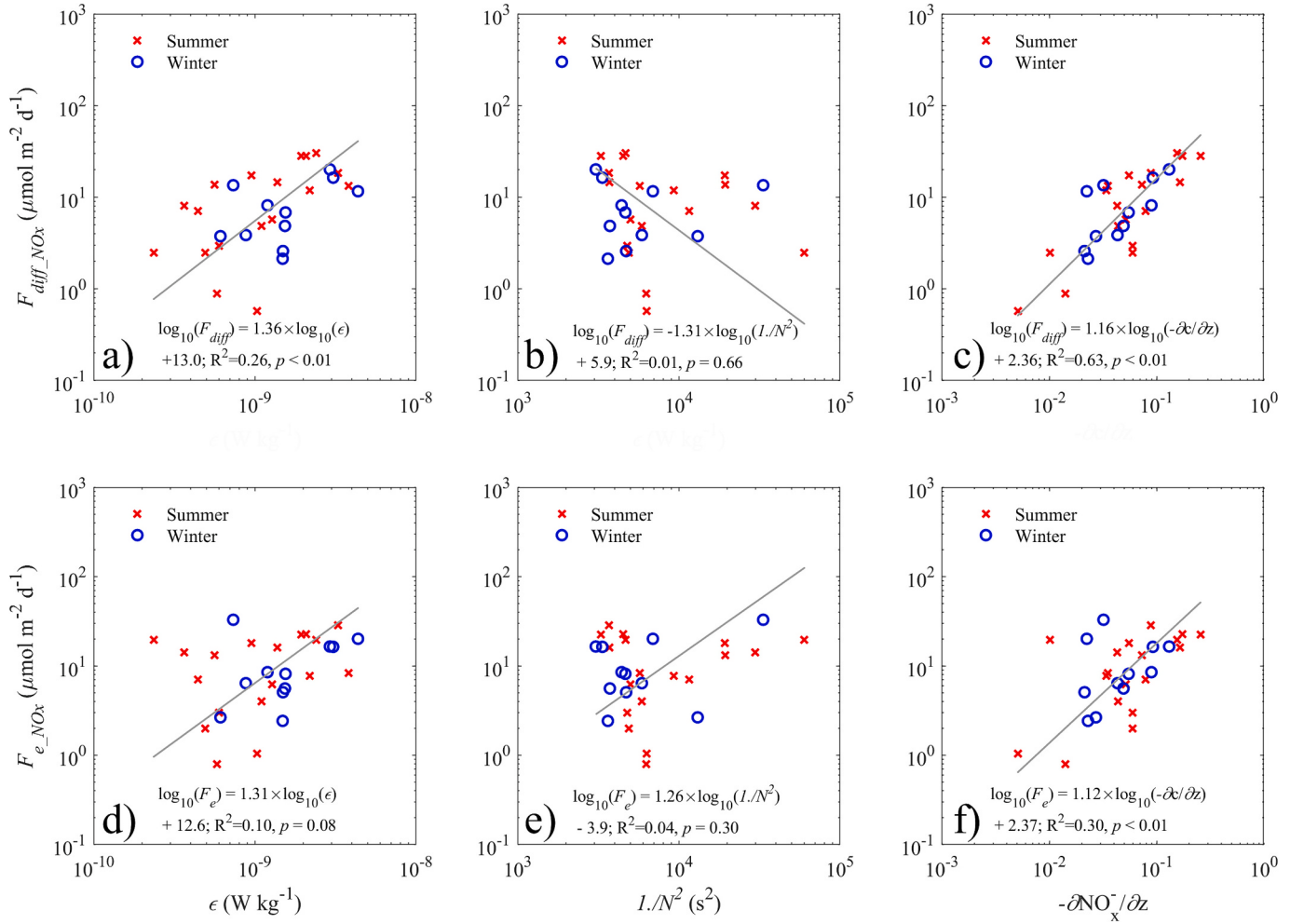
Fig. 7. Correlation analysis between diapycnal diffusive flux ( F_{\text{diff\_NOx}} ) and effective diapycnal flux ( F_{e\_NOx} ) of \text{NO}_x^- , along with the parameters \epsilon (a, d), 1/N^2 (b, e) and -\partial\text{NO}_x^-/\partial z (c, f). The texts and number denote the regression equation, coefficient of determination ( R^2 ) and the p value. Noted that the regression analysis is performed using logarithmic relationships between the fluxes and the parameters.
