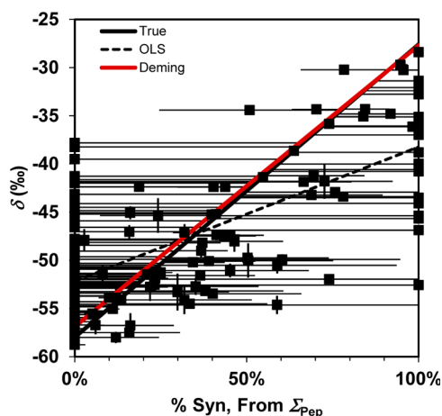
Figure 6. All values of \delta'_m plotted against the % Synechocystis peptide signal ( \Sigma\text{Pep}_{\text{Syn}}/\Sigma\text{Pep}_{\text{Total}} ). Error in \delta'_m ( \sigma_{\delta'_m} ) in most cases is smaller than the size of the symbol. Large errors in the % Synechocystis estimates are a strong function of the concentration ( \Sigma\text{Pep} ion counts). Deming regression accurately predicts the true endmembers, while OLS regression does not. See also Figure S12, Supporting Information.
