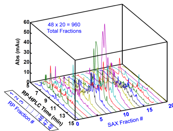
Figure 1. Protein extract obtained from a mixture of A. vinosum and Synechocystis cells, separated by SAX chromatography followed by RP chromatography. Each of the 20 fractions of the SAX dimension shows both the complexity within, and also the differences between, the adjacent fractions. Each of the RP chromatograms is divided into 48 equal time slices for collection in 96-well plates. For additional comparison of the individual RP chromatograms, see Figure S5, Supporting Information.
