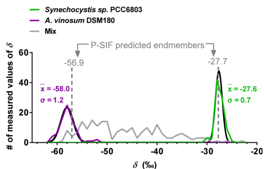
Figure 5. Histogram of values of \delta'_m for pure cultures of Synechocystis sp. PCC6803 (green line), A. vinosum DSM180 (purple line), and a mixture of the two species (solid gray line). The data for individual species are Gaussian (black lines). Regression of all values of \delta'_m for the mixture against the fraction of each species as predicted from peptide sequencing yields endmember values for \delta_{\text{Allo}} and \delta_{\text{Syn}} (gray dashed lines).
