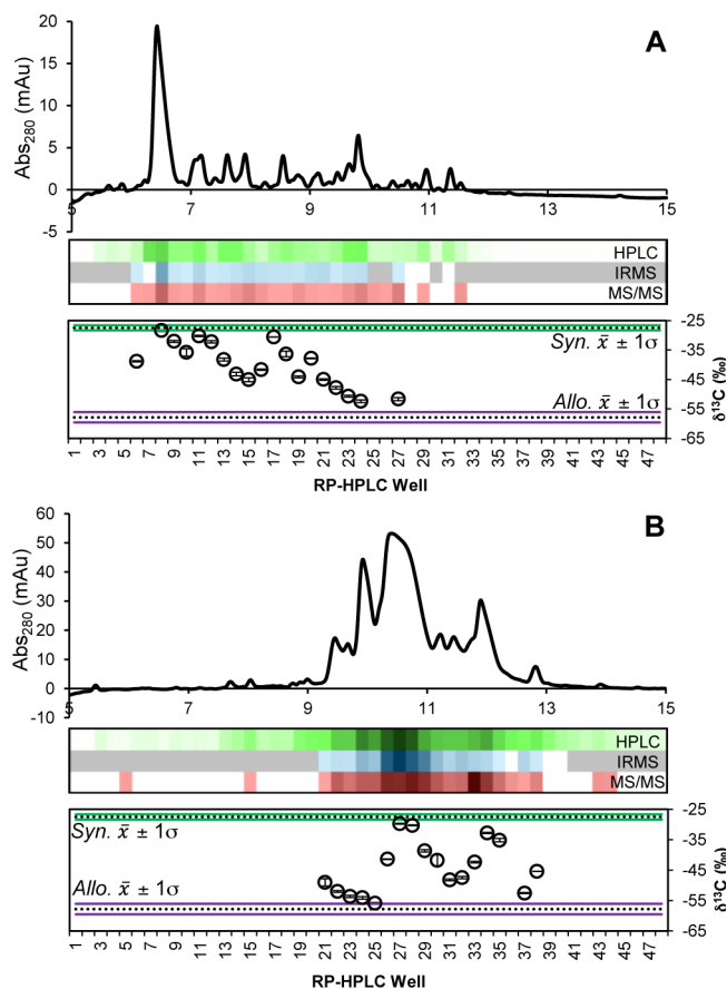
Figure 4. Comparison of protein yield and isotope data obtained from SAX.03 (A) and SAX.09 (B). The upper panel of each shows the RP-HPLC chromatogram ( A_{280} ); the middle panel shows quantification by three methods (absolute values for color scales in Figure S6, Supporting Information); and the bottom panel shows values of \delta'_m for the individual wells. Note the rapid transition from -56\text{‰} to -29\text{‰} across wells 25–27 in (B), representing <30 s of chromatography.
