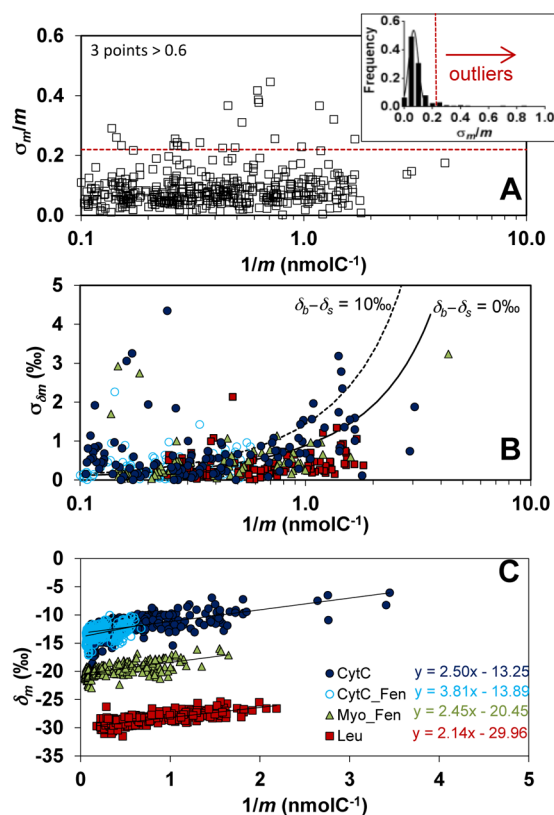
Figure 3. (A) Relative error in CO 2 combustion yields ( \sigma_m/m ); each point represents a triplicate analysis of either an amino acid or protein standard. (B) Error in values of \delta_m ( \sigma_{\delta_m} ), after removing outliers from (A) and sorted by type of standard. (C) Values of \delta_m for the same data, after removing those with \sigma_{\delta_m} > 2\text{‰} ; offsets are a function of sample size, m , and are parallel in slope regardless of \delta_s .
