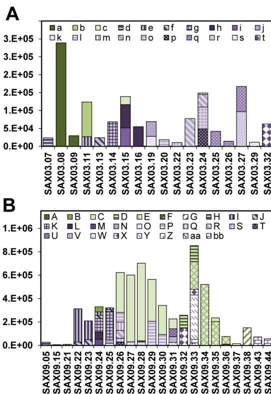
Figure 2. Protein identifications for fractions SAX.03 (A) and SAX.09 (B). Green shaded patterns are hits from Synechocystis sp. PCC6803, while purple shaded patterns are hits from A. vinosum DSM180. Protein names corresponding to the legend code letters are shown in Figure S7, Supporting Information.
