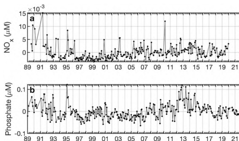
Figure 21. Long-term variability in (a) \text{NO}_x and (b) phosphate concentrations at a depth of \sim 5 m at Station ALOHA (measured using highly sensitive methods). Depicted are the anomalies (monthly mean value subtracted) of each property. Data are from Hawaii Ocean Times-series ( https://hahana.soest.hawaii.edu/hot/hot-dogs/ ).
