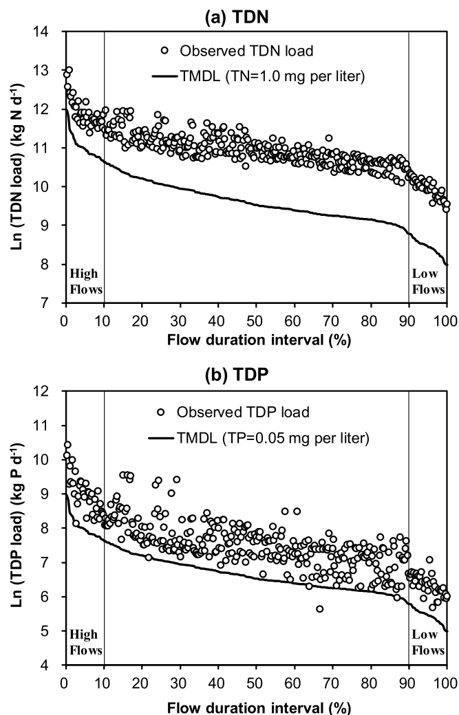
Fig. 4. The observed nutrient load into Jiangdong Reservoir in 2014, compared with the allowable total maximum daily load (TMDL) over flow regime. By adopting the load duration curves approach (USEPA, 2007), the allowable TMDLs were determined by national water quality criterion (TN = 1.0 mg L -1 , TP = 0.05 mg L -1 ) and corresponding discharge.
