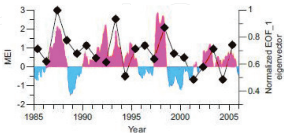
Figure 5. Variation of the eigenvector of SST EOF Mode 1 (EOF_1) in the TWS (black dots) and monthly multivariate ENSO index (MEI; shaded areas) 3 months ahead of the SST EOF_1 eigenvector during 1985–2005. The SST EOF_1 eigenvector is normalized by its maximum for the period 1985–2005. Redrawn from Hong et al. [46].
