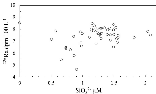
Fig. 5. The activity of ^{226}\text{Ra} vs. silicate concentration in the surface seawater in the Luzon Strait and the northern SCS slope and basin in May–July 2014.
