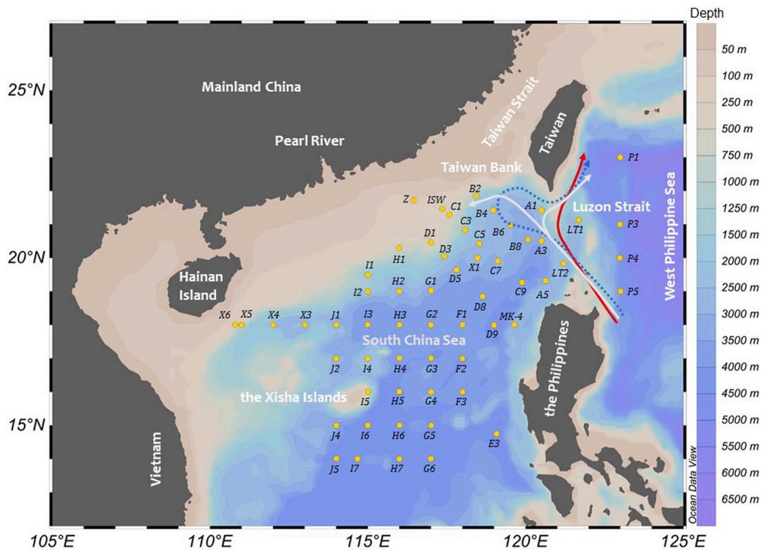
Fig. 1. Study area and sampling stations. The red, white, and dotted blue lines indicate the leaping, leaking, and looping intrusion path of the Kuroshio, respectively (Nan et al., 2011a).
