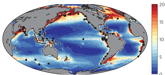
Figure 3 | Deglacial \delta^{15}\text{N} records and export flux at 100 m. Coloured shading shows a satellite-derived estimate of export production in \text{mmol C m}^{-2}\text{ d}^{-1} , according to the algorithm of ref. 48, while black circles show the locations of sediment records that have sufficient temporal resolution to be included in the deglacial analysis.
