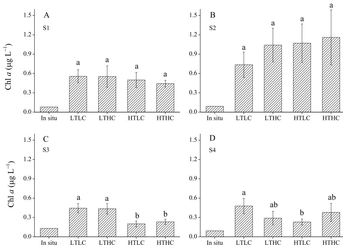
Fig. 3. Chl a concentration of surface phytoplankton assemblages in situ and in the bottle after 6 days of incubation at different experiment conditions. Different letters indicated statistically difference based on Tukey post hoc test. The values represent the mean ± standard deviation (error bar) for three replicates.
