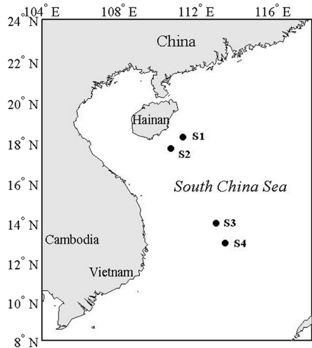
Fig. 1. Sampling stations in the western South China Sea in the cruise during autumn 2017.
