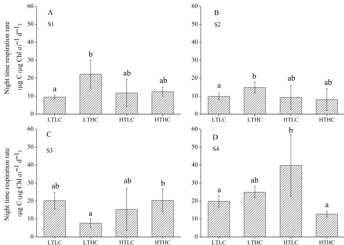
Fig. 6. Night time respiration rate of surface phytoplankton assemblages in the bottle after 6 days of incubation at different experiment conditions. Different letters indicated statistically difference based on Tukey post hoc test. The values represent the mean \pm standard deviation (error bar) for three replicates.
