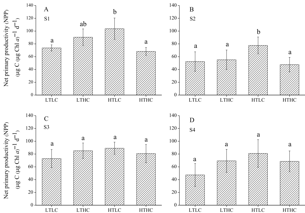
Fig. 5. Net primary productivity (NPP) of surface phytoplankton assemblages in the bottle after 6 days of incubation at different experiment conditions. Different letters indicated statistically difference based on Tukey post hoc test. The values represent the mean \pm standard deviation (error bar) for three replicates.
