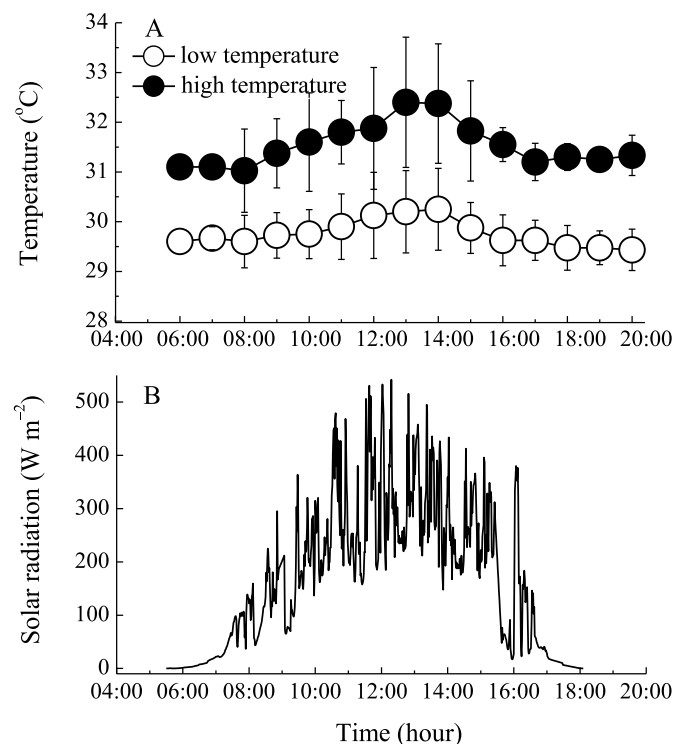
Fig. 2. Water temperature in the deck incubators for the low and high temperature treatments during the incubations, and solar radiation.
