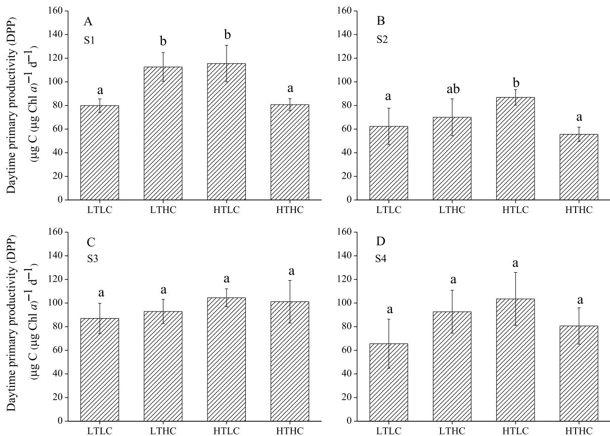
Fig. 4. Daytime primary productivity (DPP) of surface phytoplankton assemblages in the bottle after 6 days of incubation at different experiment conditions. Different letters indicated statistically difference based on Tukey post hoc test. The values represent the mean \pm standard deviation (error bar) for three replicates.
