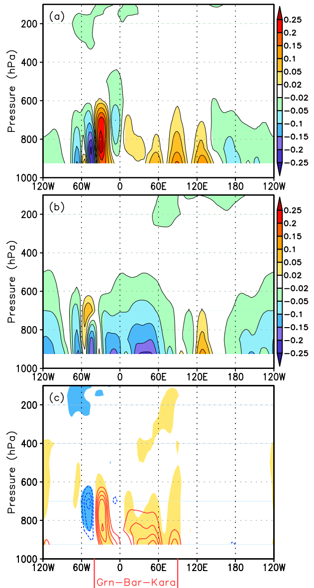
FIG. 10. As in Fig. 9, but for vertical stationary wave activity flux along the latitude of 70°N. Contour interval in (c) is 0.05 \text{ m}^2 \text{ s}^{-2} , and the shaded areas denote the 95% significance level. The two red lines mark the longitude positions of the Greenland–Barents–Kara Seas.
