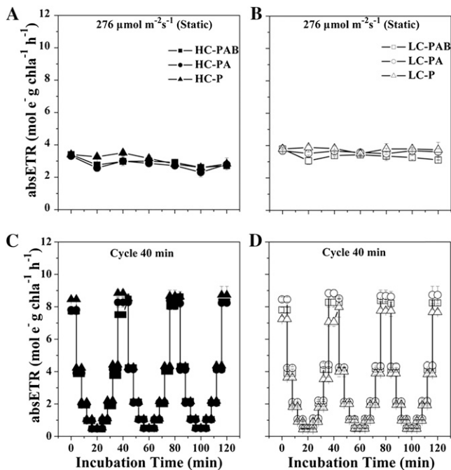
Figure 2. absETR ( \text{mol e}^- \text{g}^{-1} \text{chl a h}^{-1} ) in HC- and LC-grown cells as a function of incubation time. A, absETR under HC (A) and LC (B) conditions with constant PAR of 276 \mu\text{mol photons m}^{-2} \text{s}^{-1} . C and D, absETR under fluctuating radiation for the HC (C) and LC (D) cells at 40 min per cycle (Fig. 3). Vertical lines represent sd of triplicate incubations.
