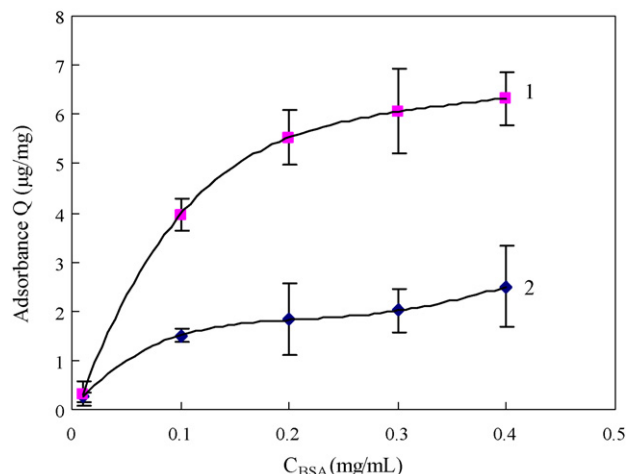
Fig. 4. Adsorption isotherms of PMIM/MWNTs (curve 1) and nPMIM/MWNTs (curve 2) to BSA. Amounts of PMIM/MWNTs or nPMIM/MWNTs: 200 mg; volume of BSA: 3 mL; time of adsorption: 3 h; vibration frequency: 150 r/min; n = 3 .
