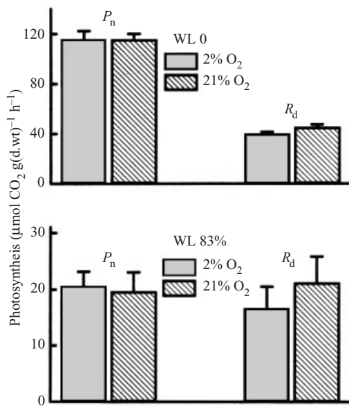
Fig. 8. Net photosynthesis ( P_n ) and dark respiration ( R_d ) of Nostoc flagelliforme in air containing ambient (21%) and reduced (2%) O_2 concentrations. Algal samples were rehydrated at 25 °C and 40 \mu\text{mol m}^{-2} \text{s}^{-1} , and measured at 770 \mu\text{mol m}^{-2} \text{s}^{-1} and 25 °C in the closed system. Bars indicate the means of 7 mats \pm SD. WL, water loss.
