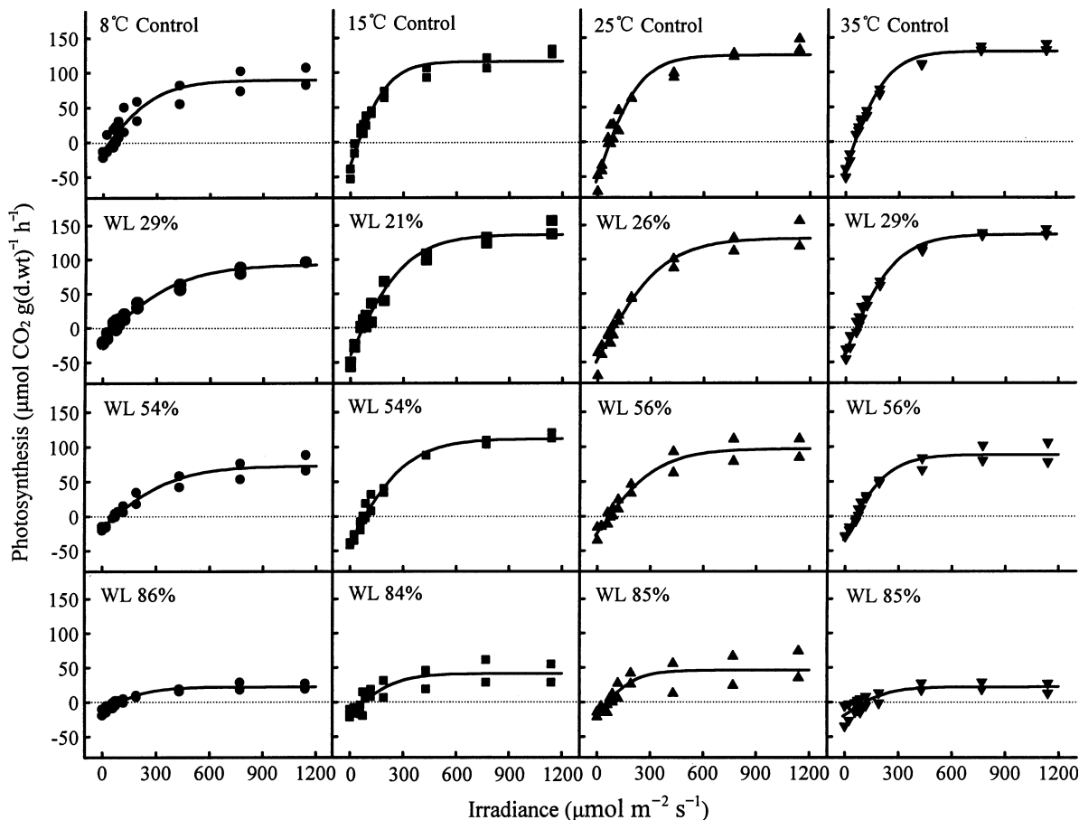
Fig. 3. Photosynthesis of Nostoc flagelliforme as a function of irradiance at various temperatures and degrees of water loss (WL). Algal samples were rehydrated at 40 \mu\text{mol m}^{-2} \text{s}^{-1} and the experimental temperatures (8, 15, 25 and 35 °C), and measured in the open system. Less than 8% water was lost during each measurement. Wet samples (0% water loss) were used as control. Each P-I curve shows the mean from two separate mats.
