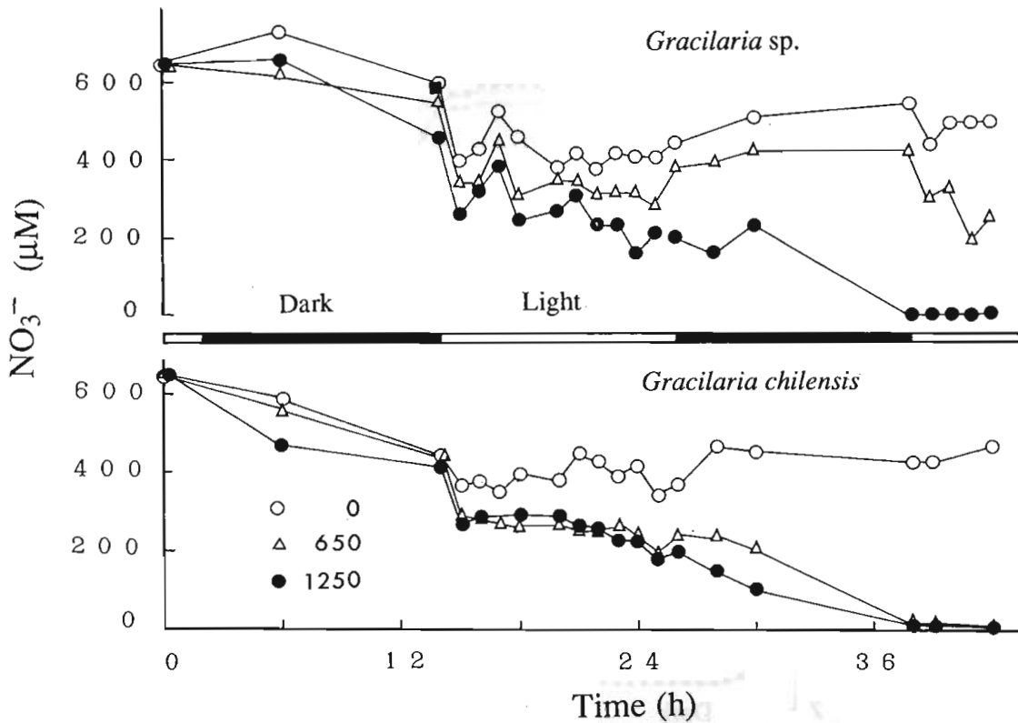
Fig. 3. \text{NO}_3^- concentrations in N- and P-enriched cultures of Gracilaria sp. and G. chilensis aerated with air + 0 ppm \text{CO}_2 , air + 650 ppm \text{CO}_2 and air + 1250 ppm \text{CO}_2 . Measured from the 6th day after the initiation of the experiment.
