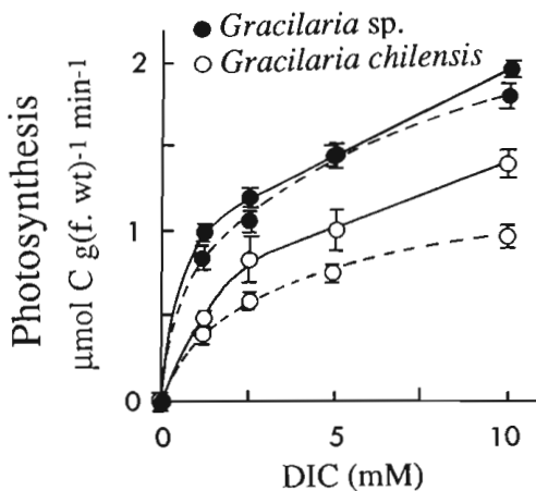
Fig. 4. Photosynthetic inorganic carbon uptake as a function of dissolved inorganic carbon (DIC) concentration of seawater in Gracilaria sp. and G. chilensis pre-cultured for 15 days with air (solid line) and air + 1250 ppm \text{CO}_2 (dotted line). Measured at 20 °C, 300 \mu\text{mol photon m}^{-2} \text{s}^{-1} . Means \pm SD ( n = 3 ).
