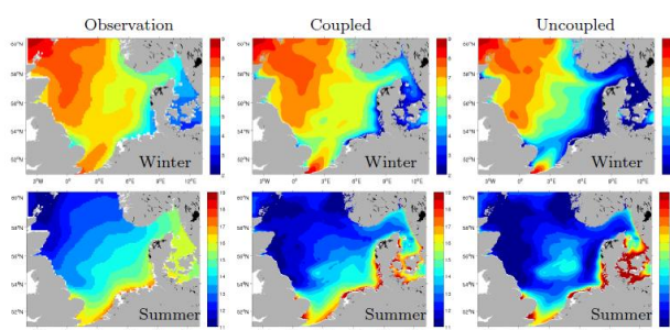
Figure 1. Fourteen years mean SST ( ^{\circ}\text{C} ) of observations (Janssen
